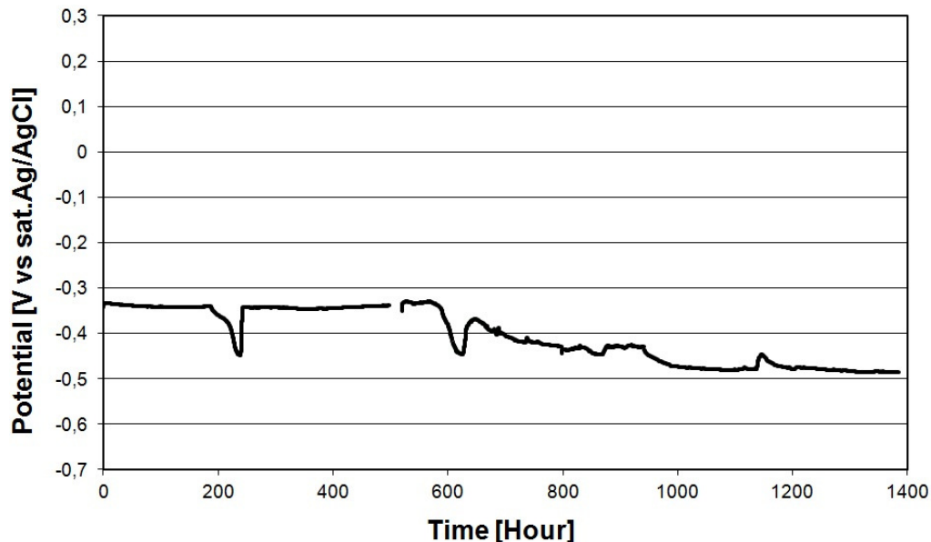
Figure 3: Galvanostatic test, during 1400 uur at 5\mu\text{A}/\text{cm}^2 .
