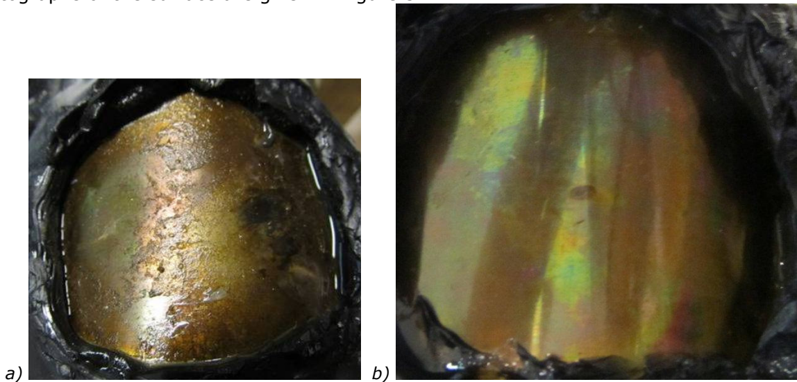
Figure 5: The surface after testing, before (a) and after 9b) removing the corrosion product with a cloth.
